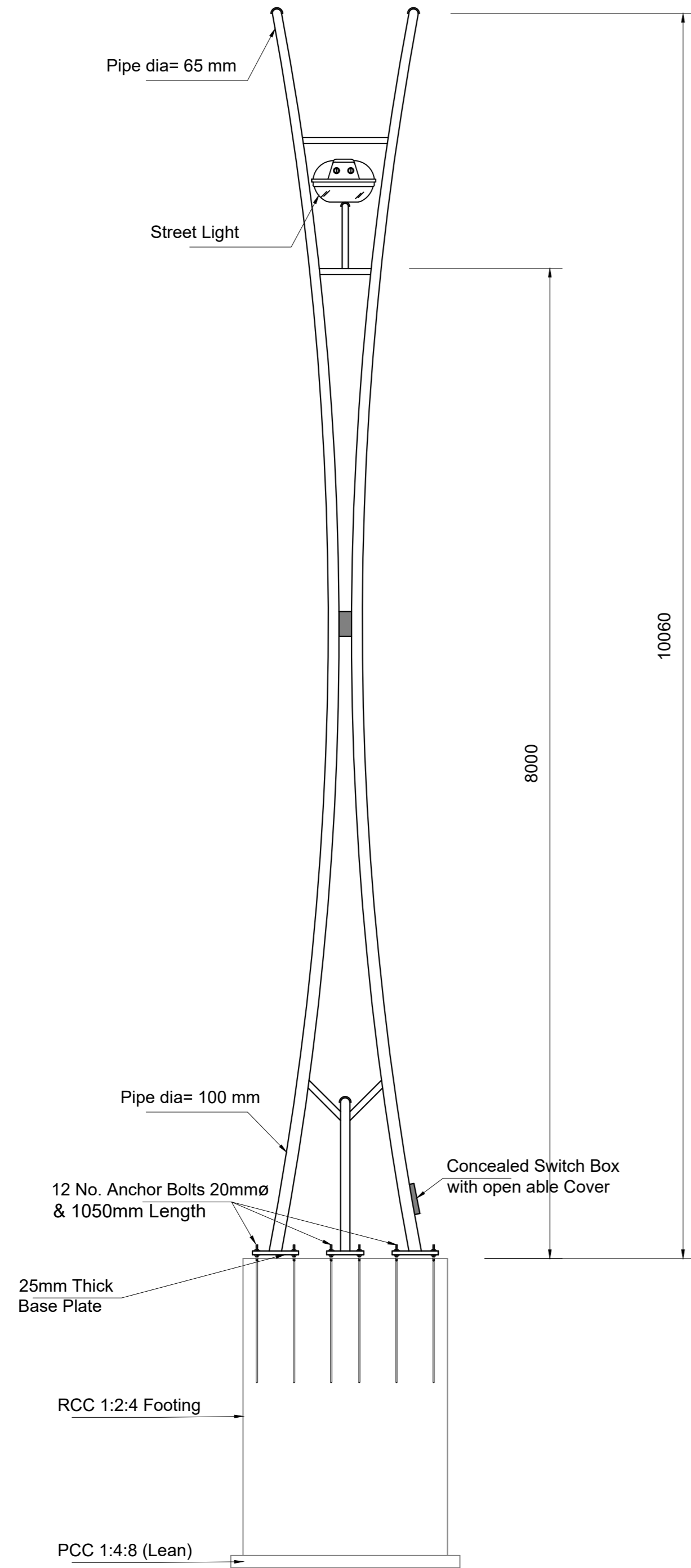
STREET LIGHT POLE FRONT VIEW
