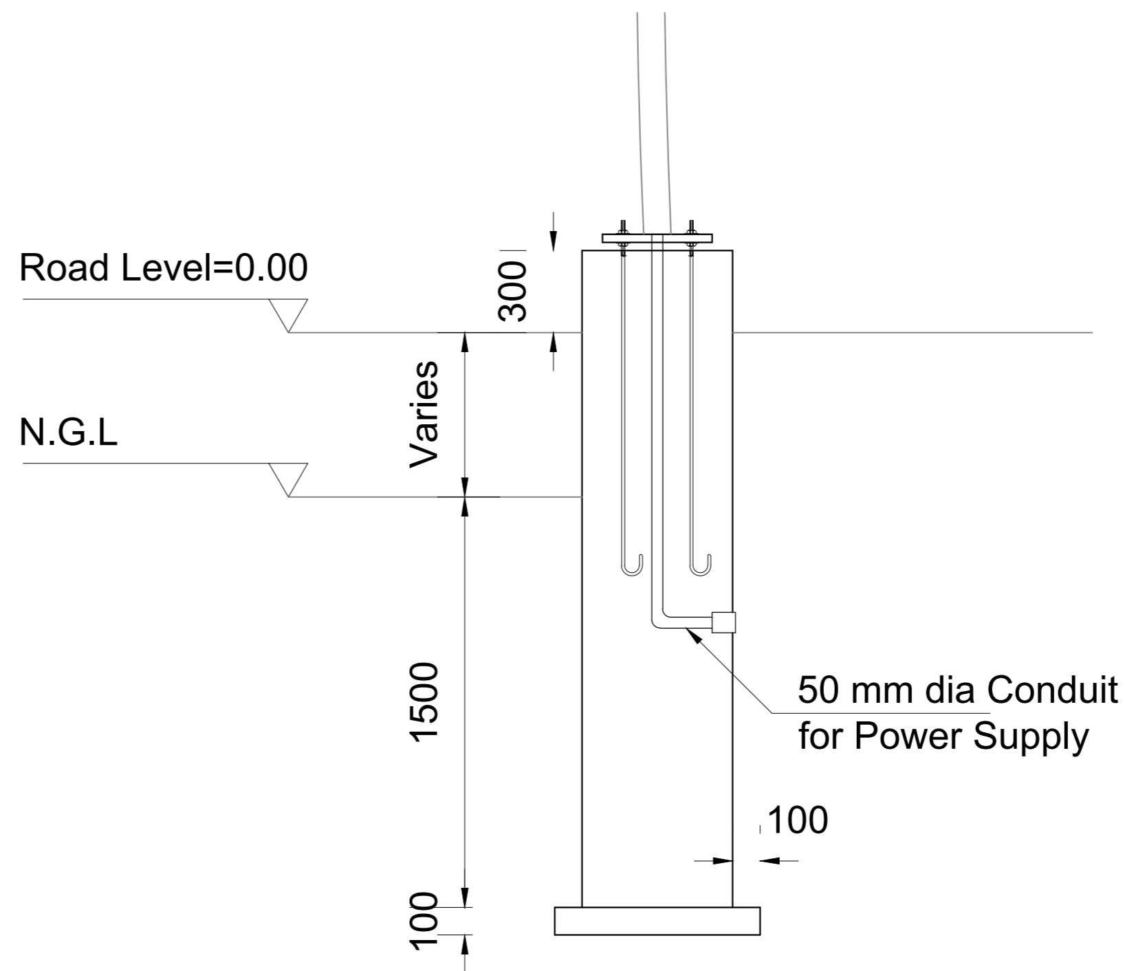
Footing Side View
