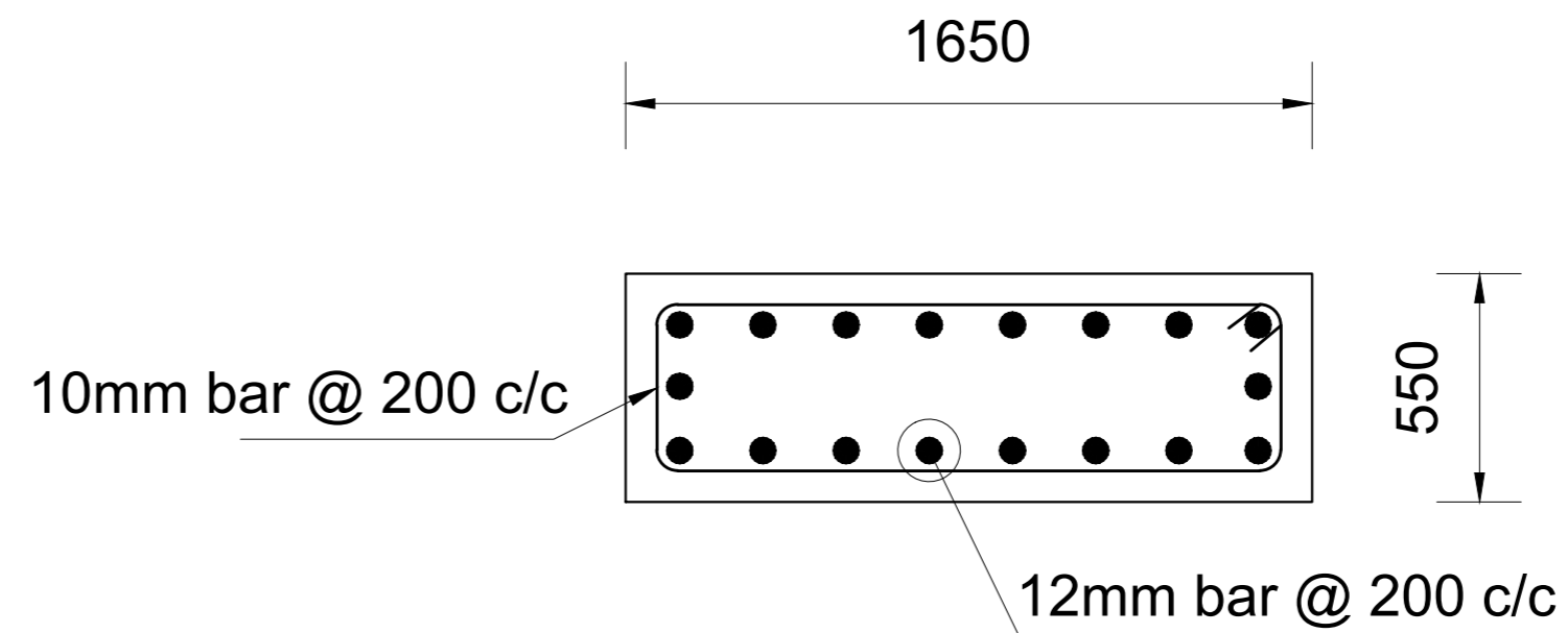
Footing Sectional Plan.
