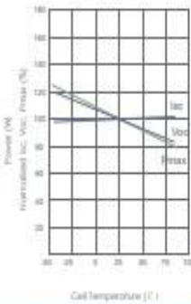
Temperature Dependence of Isc, Voc, Pmax
