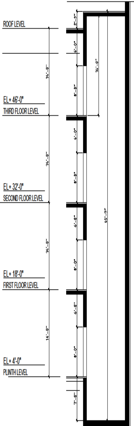
SECTION LIFT 2
