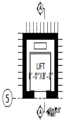
3 PLAN AT FIRST FLOOR (EL. +1'-0")
