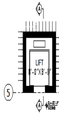
4 PLAN AT SECOND FLOOR (EL. +3'-0")
