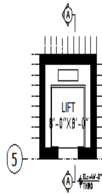
1 PLAN AT THIRD FLOOR (EL. +4'-0")
