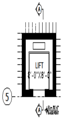
1 PLAN AT BASEMENT (EL. -1'-0")
