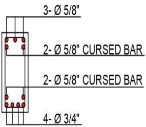
SECTION B-B ROOF BEAM -1 (12\"X24\")
