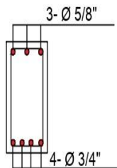
SECTION B1-B1 ROOF BEAM -2 (13.5\"X24\")
